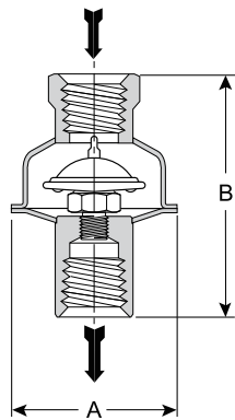
WMT-1疏水阀
